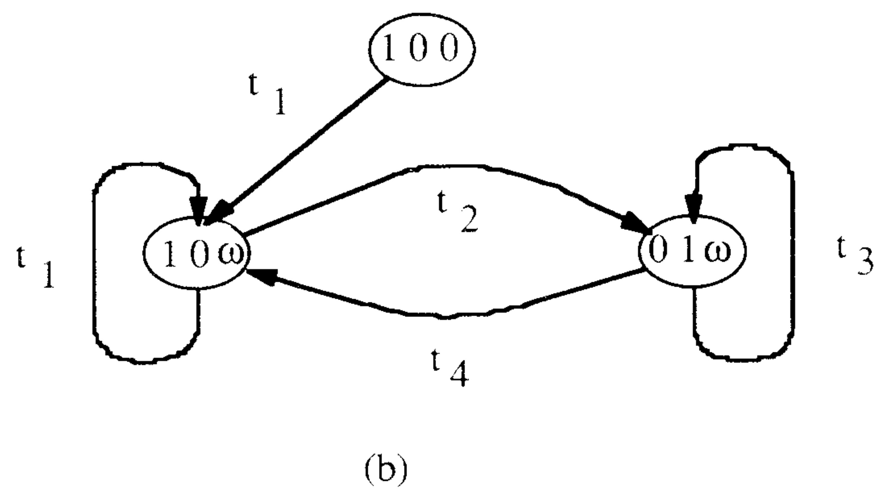
Fig. 4.3 (a) The coverability tree for both Petri nets shown in Fig. 4.2(a) and 4.2(b), and (b) the coverability graph for the two nets shown in Fig. 4.2(a) and 4.2(b).
